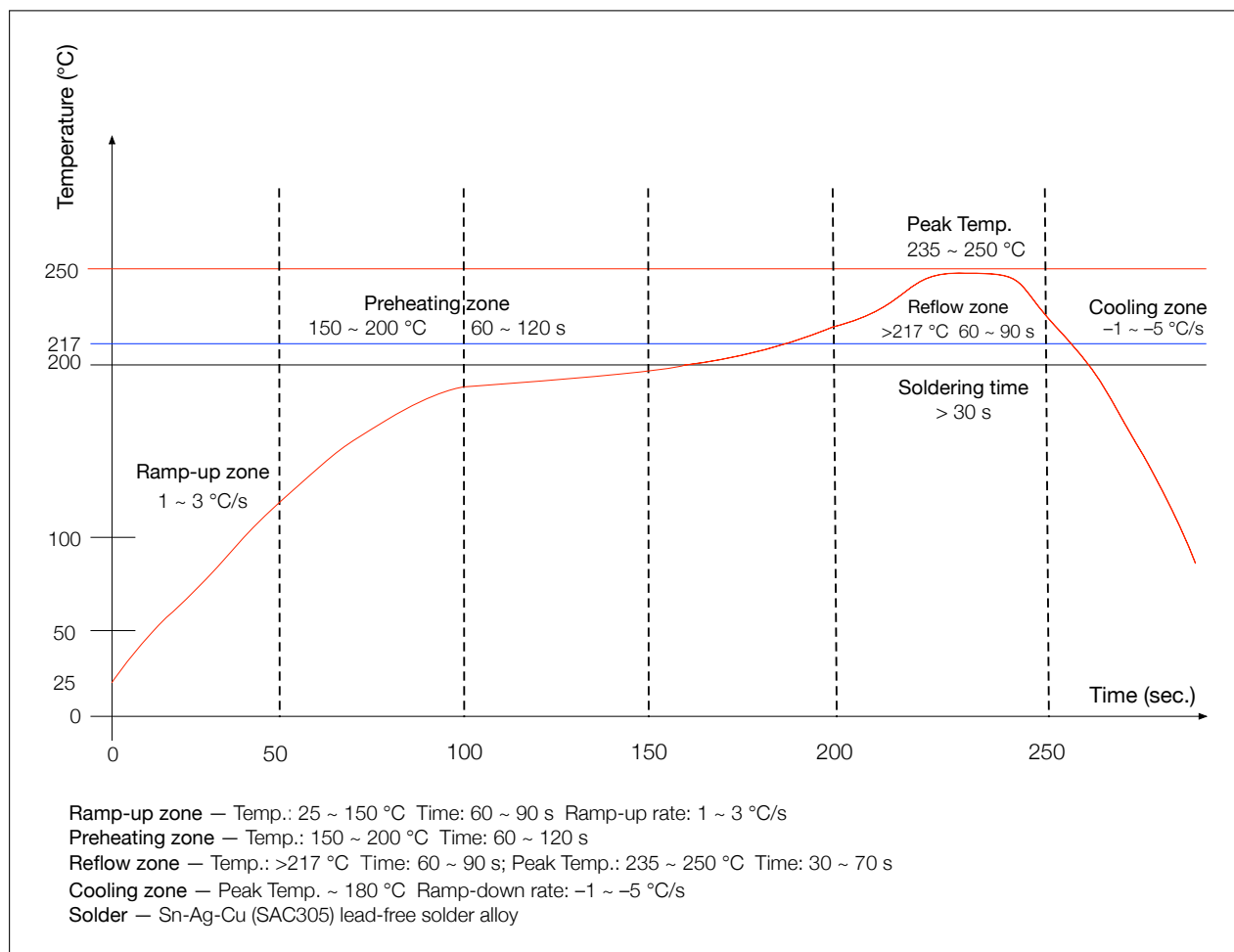
Figure 13: Reflow Profile
